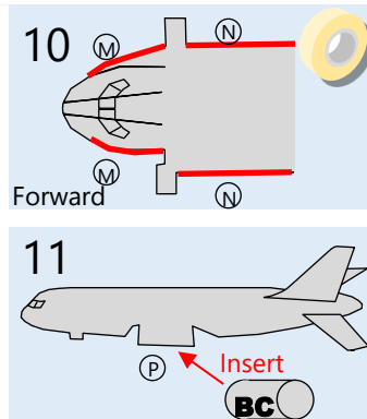
10 | Apply tape (or glue) to adhere the FG edges together: M > M | N > N .
