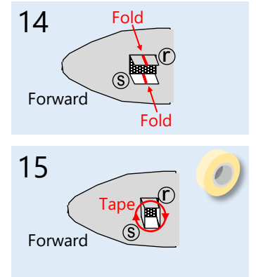
14 | Fold along the red line on the following FG tabs as indicated: r , s .
